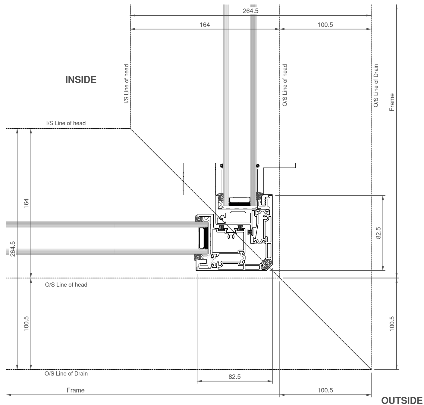
Corner Opening HORIZONTAL SECTION
